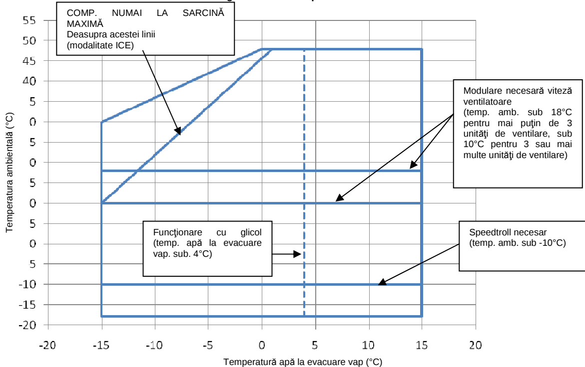
Figura 2 – Limite operative
