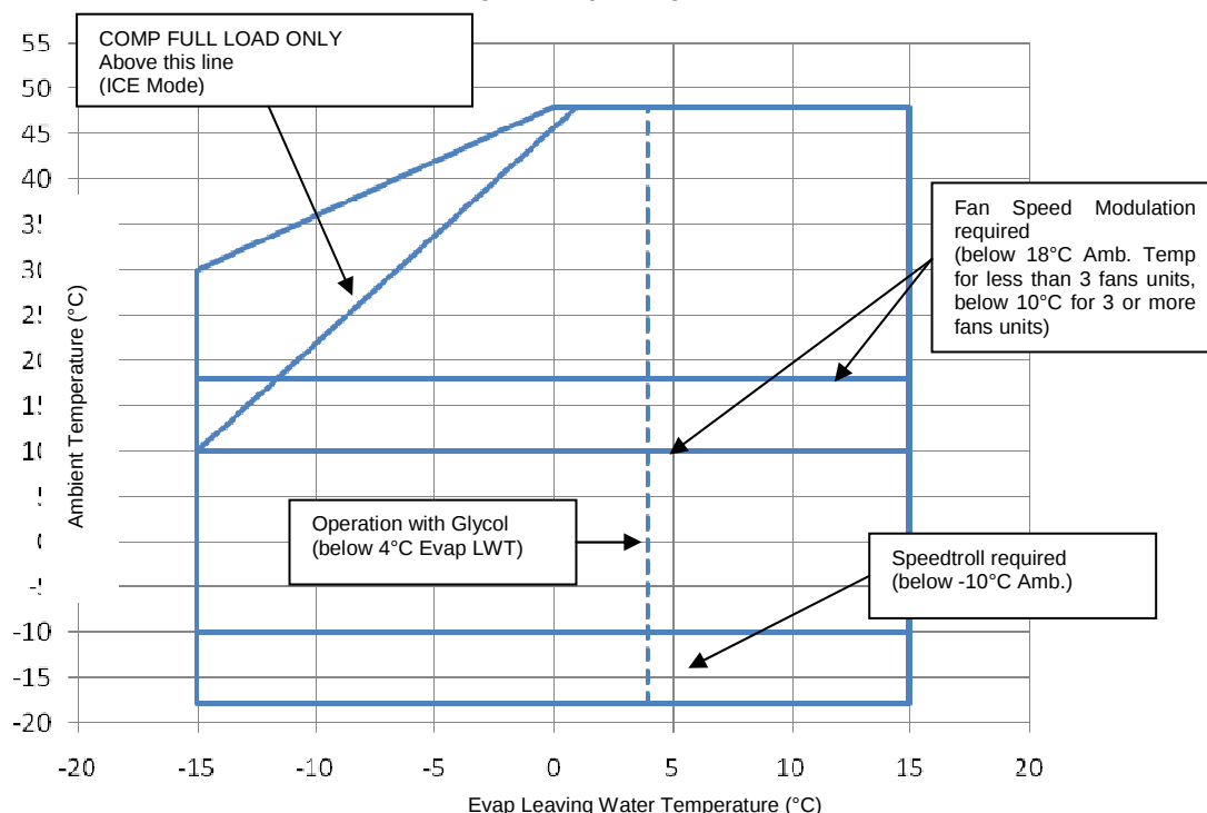
Figure 2 - Operating limits
