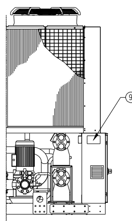
Figure 1 - Description of the labels applied to the electrical panel
